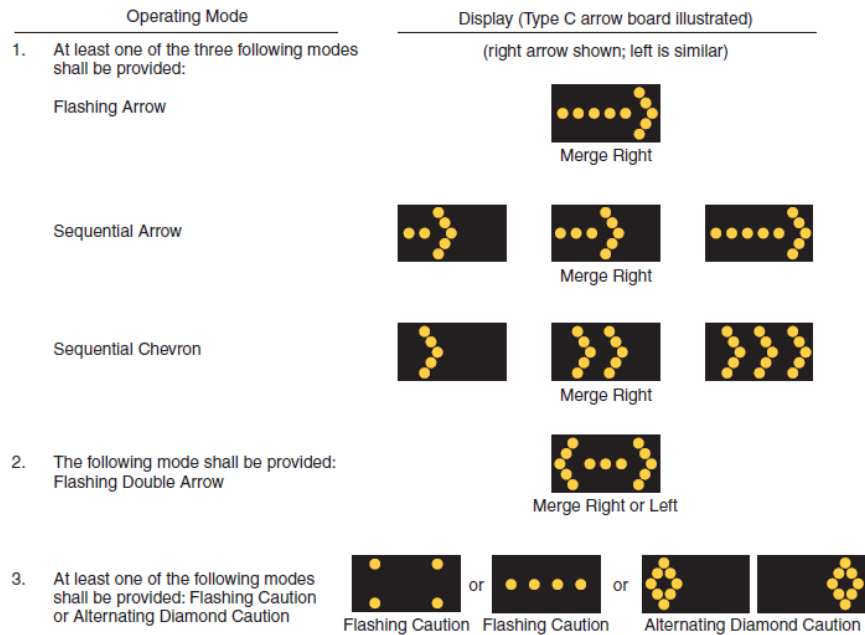
Figure 6L-3. Advance Warning Arrow Board Display Specifications
